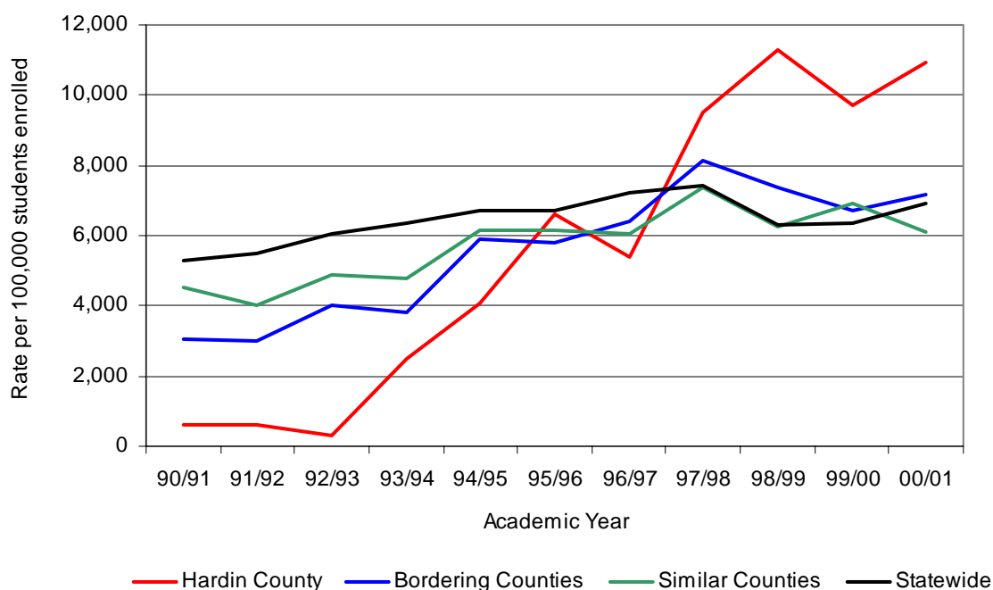
Figure 21 Suspension Rates, 1990/1991-2000/2001
