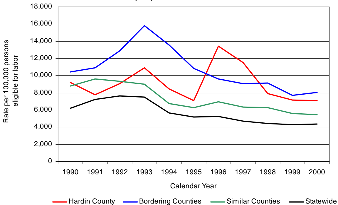
Figure 25 Unemployment Rates, 1990-2000
